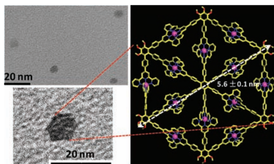
Figure 4. (left) TEM images of [\text{T6}_1\text{-Cd}_{12}\text{-T3}_6] on a carbon-coated Cu grid. (right) Representative energy-minimized structure of [\text{T6}_1\text{-Cd}_{12}\text{-T3}_6] .
