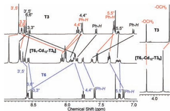
Figure 2. ^1\text{H} NMR spectra (500 MHz) of ligands T3 and T6 in \text{CDCl}_3 and [\text{T6}_1-\text{Cd}_{12}-\text{T3}_6] in \text{CD}_3\text{CN} .
