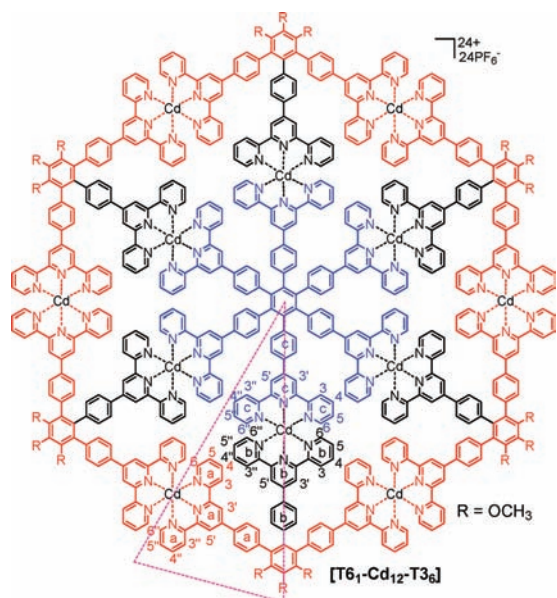
Figure 1. Structure of the supramacromolecular spoked wheel [\text{T6}_1-\text{Cd}_{12}-\text{T3}_6] ; the triangle denotes the smallest subunit.
